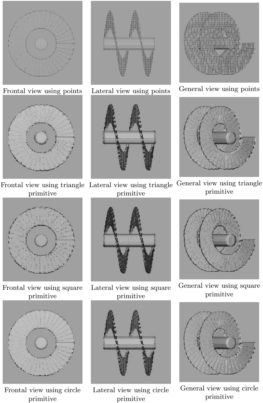
Figure 5: Comparison of the visualization with points and three primitives, triangle, square and circle, to render the splats.
